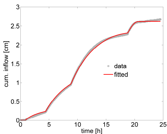
Fig. 1: Measured and fitted cumulative inflow data of ethanol for the LS material.
